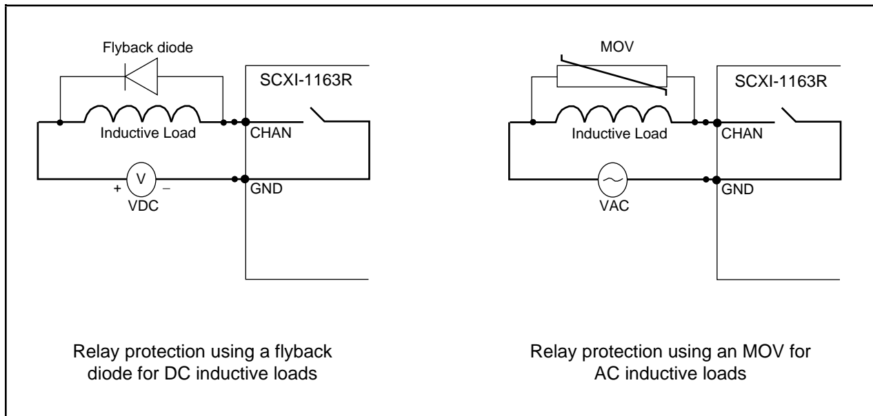
Figure 3-3. Relay Protection When Switching Inductive Loads
